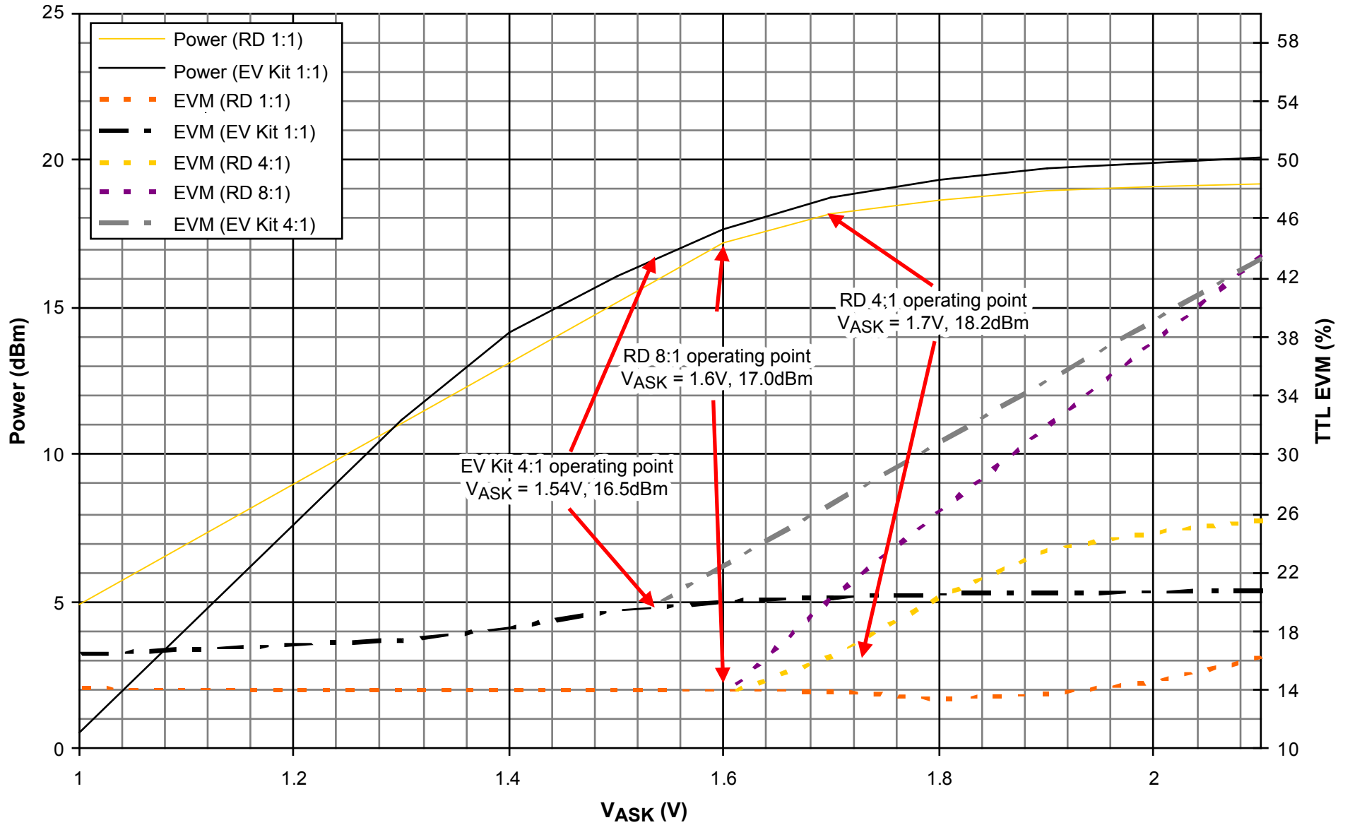
Power and EVM vs. V ASK Multiple VSWRs
