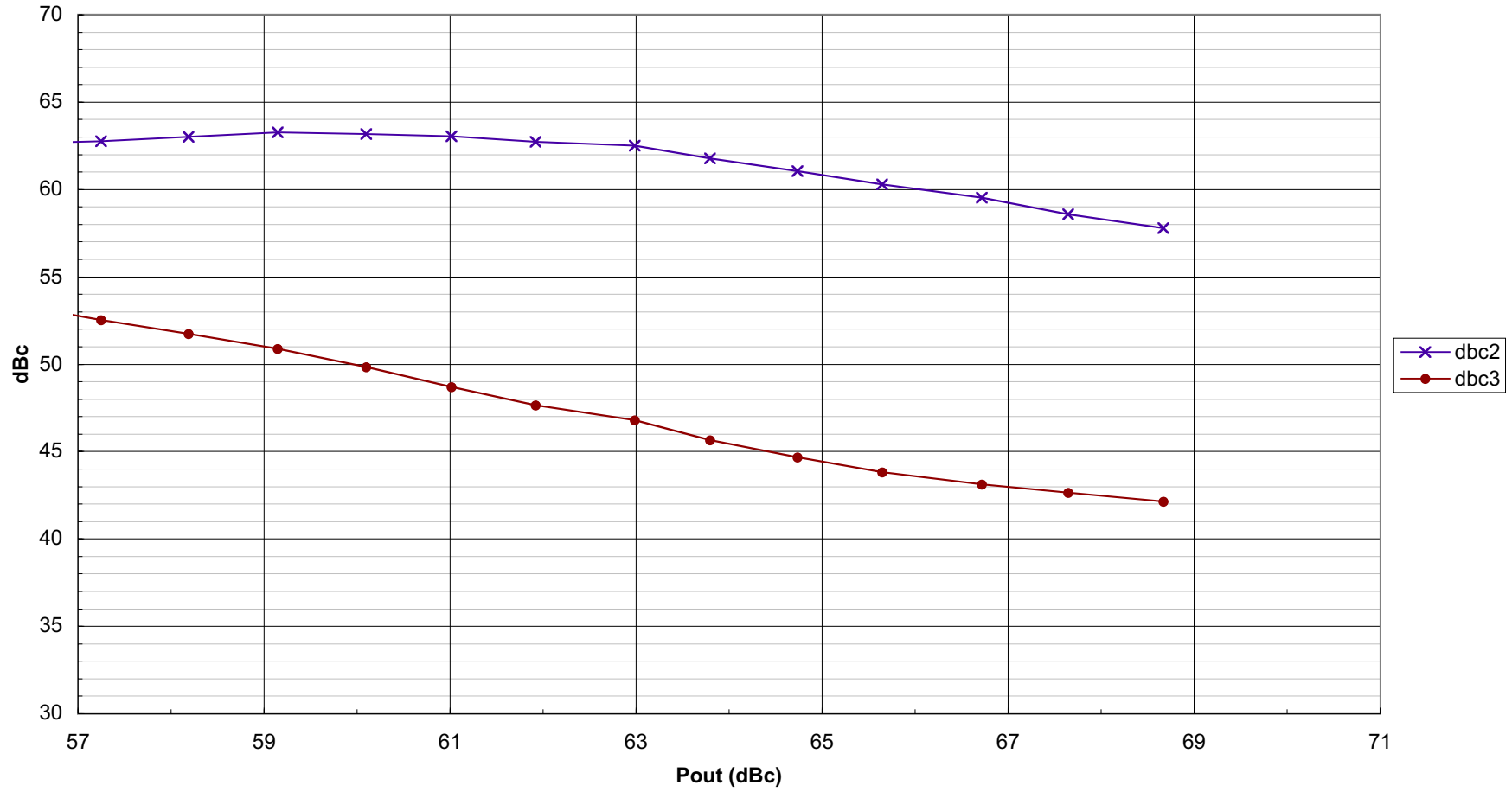
2nd 3rd Harmonic vs. Pout MAX3509 65MHz 2:1 Pin=33dBmV
