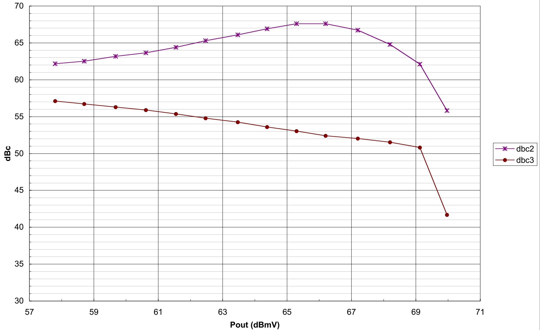
2nd 3rd Harmonic vs. Pout MAX3509 22MHz 2:1 Pin=34dBmV
