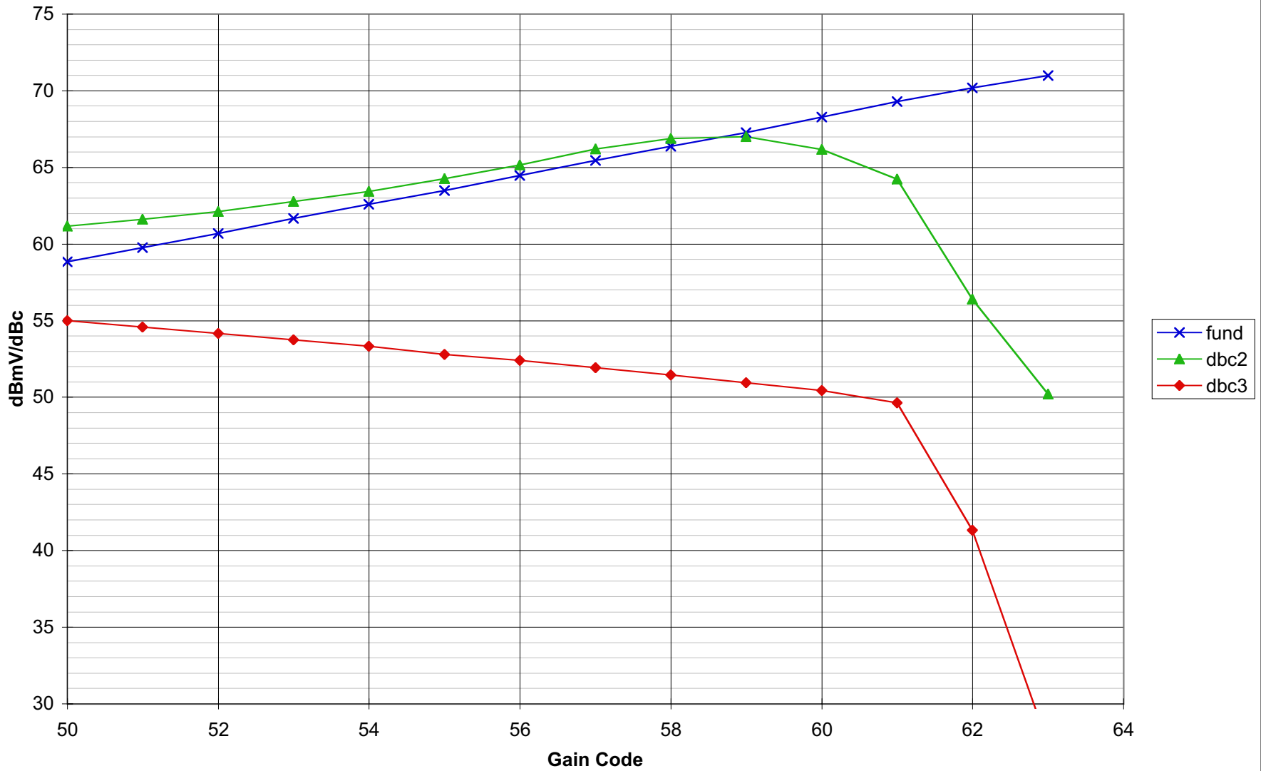
Pout, Harmonics vs. Gain Code MAX3509 22MHz 2:1 Pin=35dBmV
