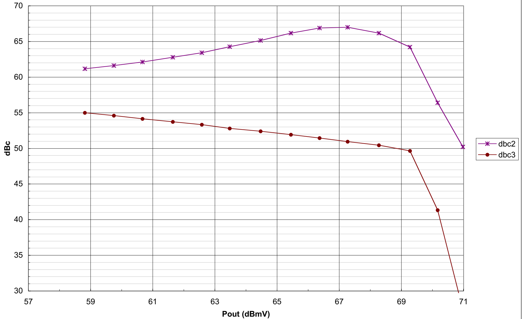
2nd 3rd Harmonic vs. Pout MAX3509 22MHz 2:1 Pin=35dBmV
